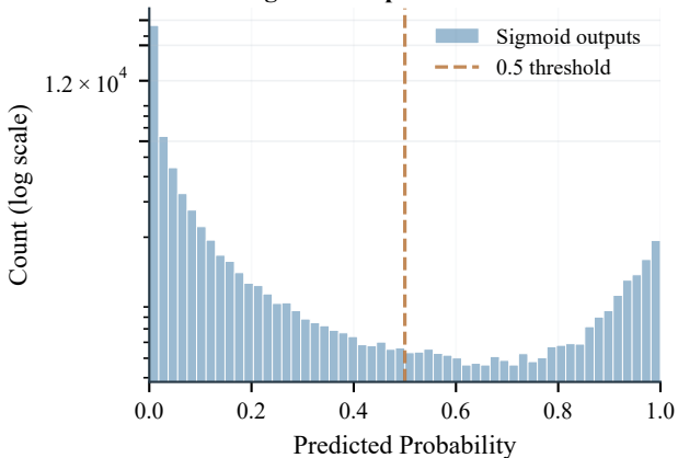
Sigmoid Output Distribution
